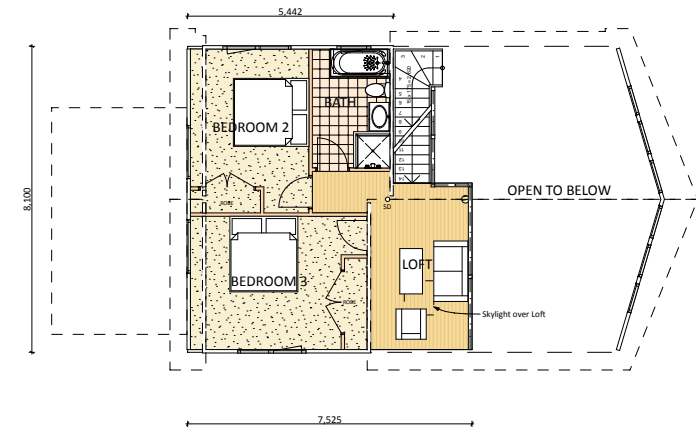
Loft Floor Plan
